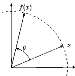
A \in SO(2, \mathbb{R})
