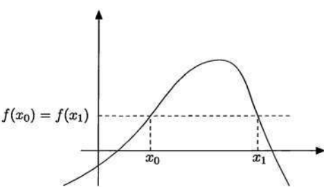
Application non injective
